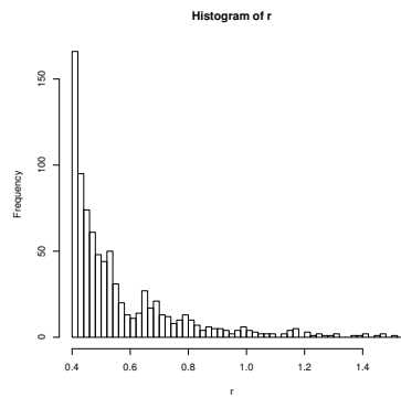
Fig. 4. Histogram of pagerank scores for Aleph predicates
